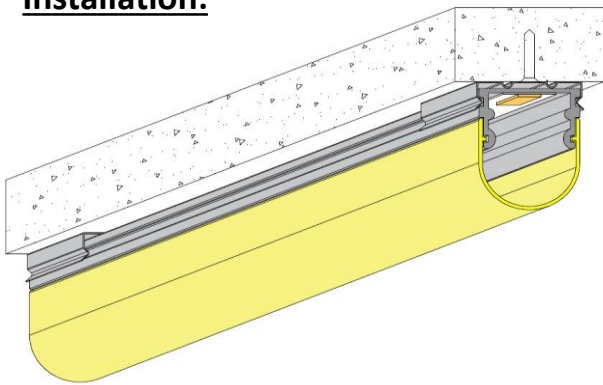
Surface Mount With Mounting Clips
