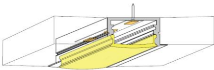
Recessed Mount With Mounting Clip
