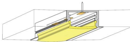
Recessed Mount Without Mounting Clip
