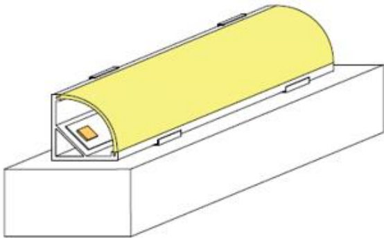
Surface Mount Without Mounting Clip
