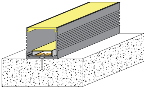
Surface Mount Without Mounting Clip
