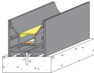
Surface Mount without Mounting Clips
