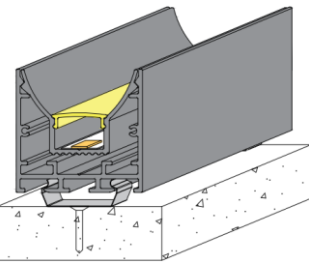
Surface Mount with Mounting Clips
