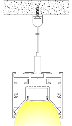
LH99-CN180 Connector
