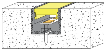
Recess Mount without Mounting Plate
