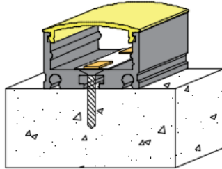
Surface Mount without Mounting Clips
