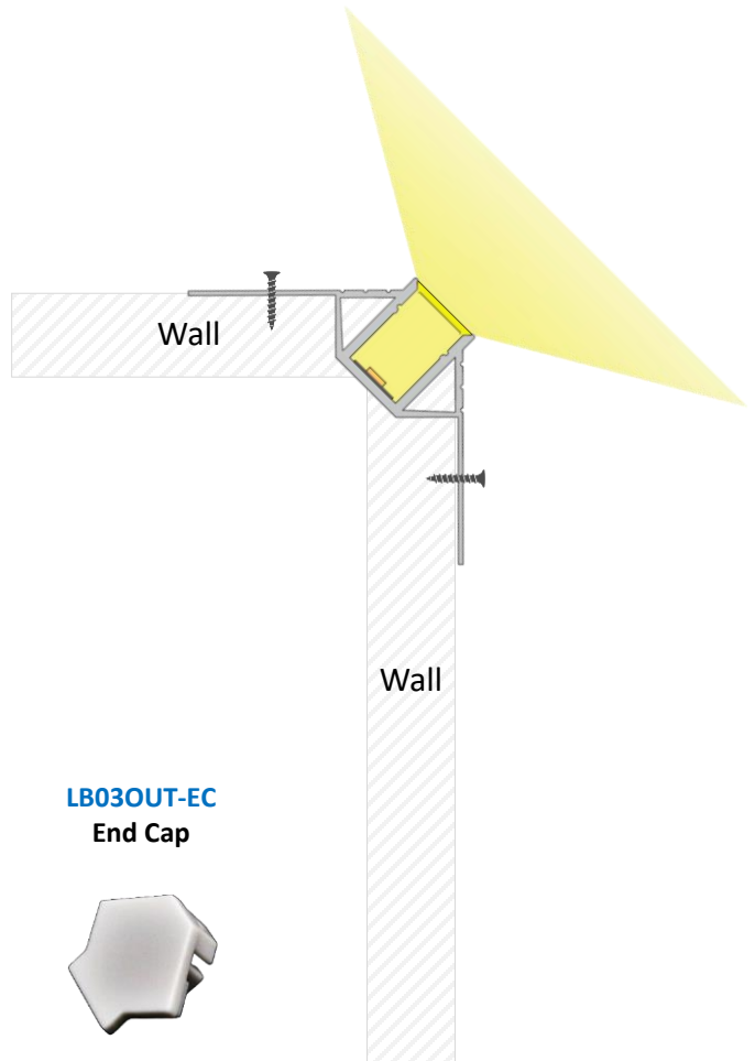
LB03OUT + LB03-SL Satined Lens
