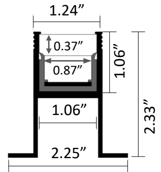
Cross Section:
